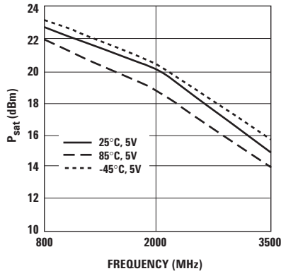
Figure 11. P_{sat} vs. Frequency. ( P_{in} = 0 \text{ dBm} , V_d = 5V )
