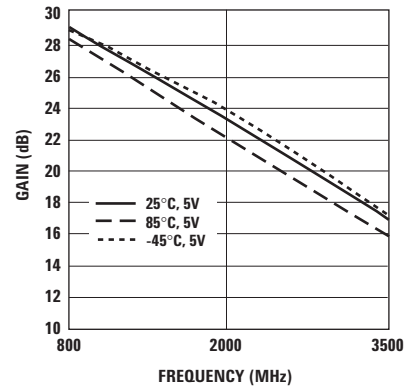
Figure 15. Gain vs. Frequency. ( P_{in} = -10 \text{ dBm} , V_d = 5V )
