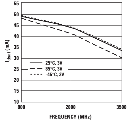
Figure 12. I_{dsat} vs. Frequency. ( P_{in} = 0 \text{ dBm} , V_d = 3V )
