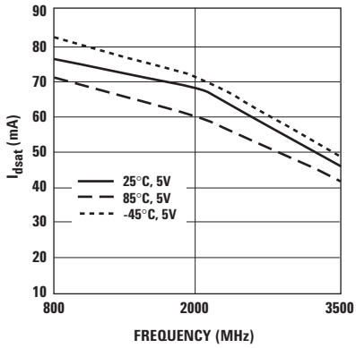
Figure 13. I_{dsat} vs. Frequency. ( P_{in} = 0 \text{ dBm} , V_d = 5V )
