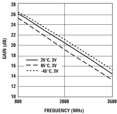
Figure 14. Gain vs. Frequency. ( P_{in} = -10 \text{ dBm} , V_d = 3V )
